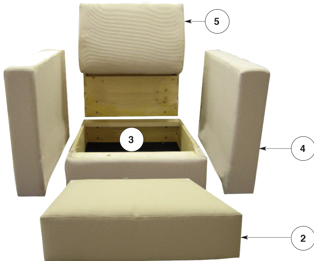
F. Strip off the fabric from the Back frame. Using a Philips screw driver, unscrew the four screws and washers to detach the Back cushion from the Back frame.
