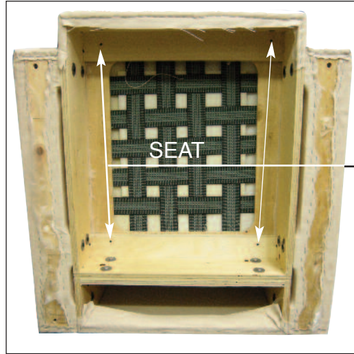
C. Using a Philips screwdriver, unscrew the four wood screws to detach the Upholstered Seat Cushion. (2)
