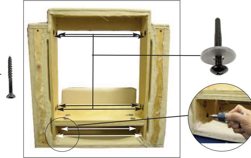
D. Using a Philips screwdriver, unscrew the eight screws and washers to detach the Arms (4) from the seat/back frame Use a snub nose Philips screwdriver to unscrew the four screws and washers indicated by white arrows
