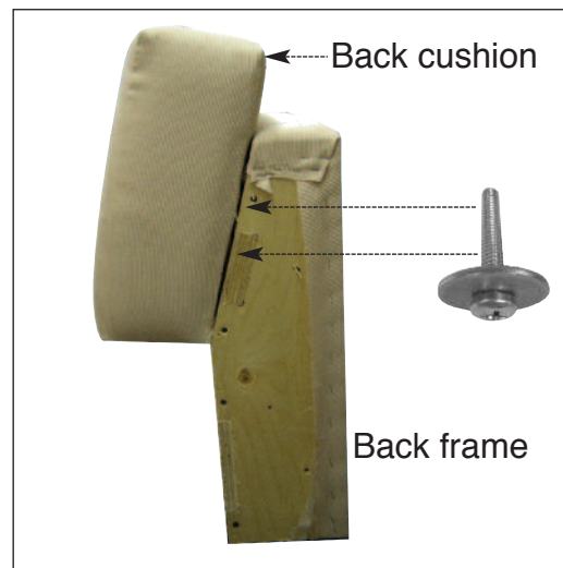
F. Strip off the fabric from the Back frame. Using a Philips screw driver, unscrew the four screws and washers to detach the Back cushion from the Back frame.
