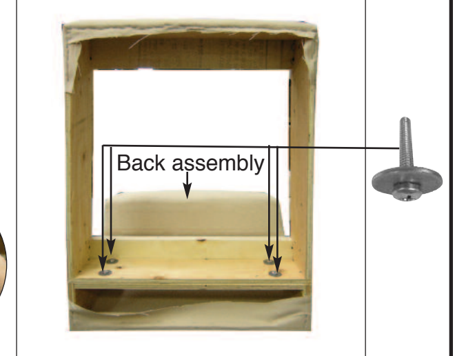
E. Using a Philips screwdriver, unscrew the four screws with washers, to detach the back assembly from the Seat frame (3)
