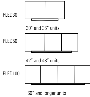
Wall Mount
