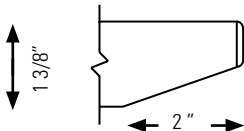
Edge Detail - Conference Tables
