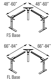
Extended Range 90° Base, Equal Sides*
