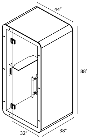
Exterior Dimensions
