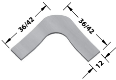
Gallery Corner Transaction Top - 1½" thick
