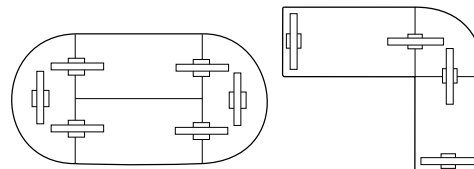
Figure 9 - 90° Leg Connections
