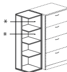
End Shelf - LEFT 52.5"/53" High**
