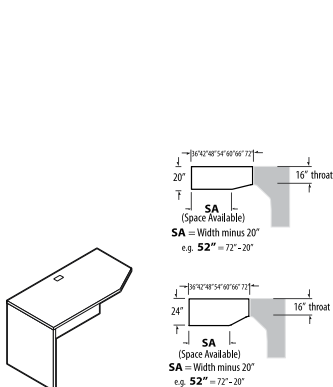
Space Saver Return - LEFT
