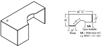
Left Extended Corner, 24" Throat Freestanding
