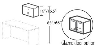
Closed Front Overhead Storage* with Doors - 16"/16.5"H*
