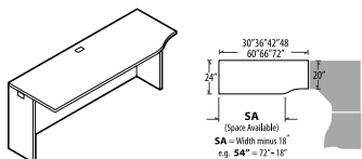
24" Deep Space Saver Connectable Table
