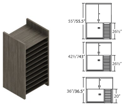
Vertical Pigeon-Hole Storage
