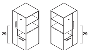
LEFT RIGHT 52" H Storage Tower w/Wardrobe, Shelf, Recycling and Bookshelf at 29" H
