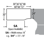
30" Deep Space Saver Connectable Table w/Wall Access
