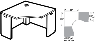
5-Sided Corner
