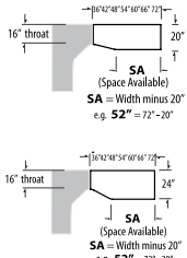
Space Saver Return - RIGHT
