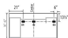
Straight Front
