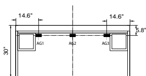
Freestanding HA
