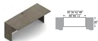
30" Deep Connectable Table
