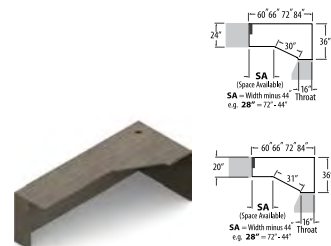
Extended Corner, 16" Throat - RIGHT*
