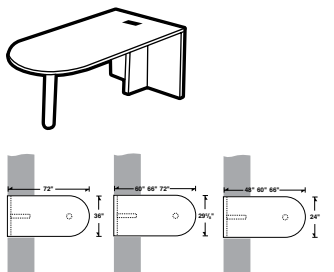
"D" Island - Full End Panel & Post (T-Base)
