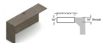
Flush Return - LEFT*
