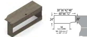
24" Deep Space Saver Connectable Table w/Wall Access - LEFT*
