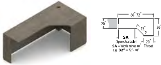
Extended Corner, 20" Throat - RIGHT
