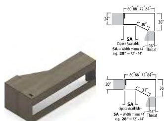
Extended Corner w/Wall Access, 16" Throat - RIGHT
