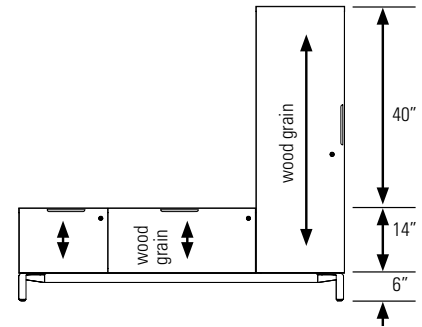
Low storage with 54" high storage on undercarriage
