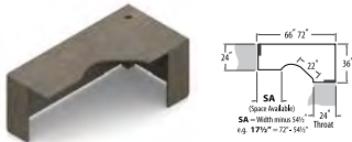
Extended Corner, 24" Throat - RIGHT
