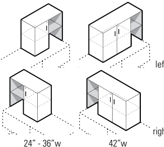
Stack-On Mixed Storage Cabinet*
