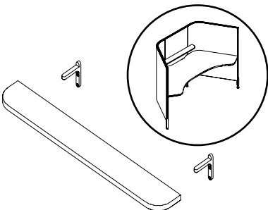
HXARWS Rear Wall Shelf Height: 3/4" Depth: 4.5" Width: 32.5" • Laminate NOTE : Not compatible with Ceiling Feed Pole or any monitor mounts.
