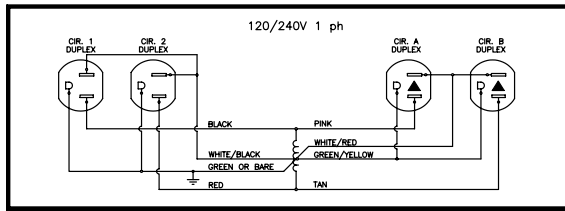
4-2-2 Wiring Schematic 8-Wire Shared Neutral "2+2" – 2 Utility circuits, 2 dedicated
