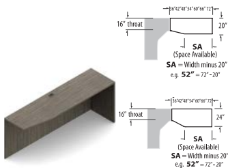
Space Saver Return - RIGHT
