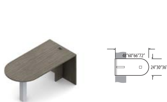
"D" Island - Full End Panel and Monopost (T-Base)
