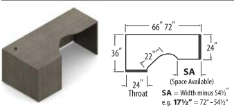
Extended Corner, 24" Throat Freestanding - LEFT
