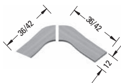
2 Piece Gallery Corner Transaction Top - 1" Thick
