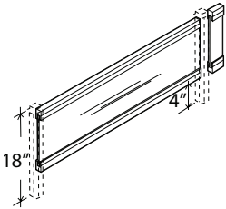
Raised Glazed Panel - 18" High
