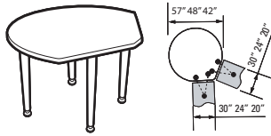
Round Wedge 120° Table
