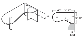
Extended Corner "P" Island Full End Panel & Post (T-Base) - LEFT
