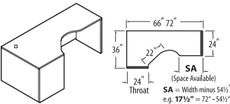
Extended Corner, 24" Throat Freestanding - LEFT
