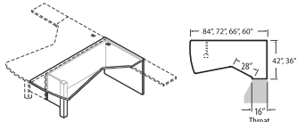
Extended Corner Island Flush Modesty and Post - LEFT*
