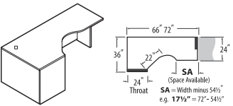
Extended Corner, 24" Throat - LEFT
