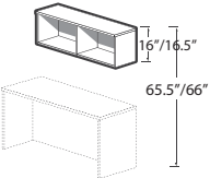
Open Front Overhead Storage 16"/16.5" High, 60" Wide
