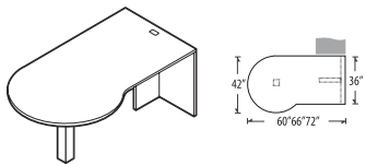
"P" Island - Full End Panel and Post (T-Base) - RIGHT*
