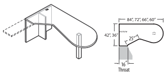
Extended Corner "P" Island Full End Panel & Post (T-Base) - RIGHT
