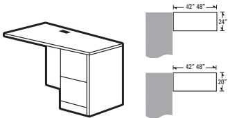
Full to Floor Flush Return - RIGHT*
