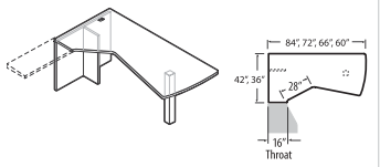
Extended Corner Island Full End Panel & Post (T-Base) - RIGHT
