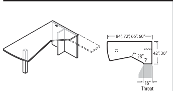
Extended Corner Island Full End Panel & Post (T-Base) - LEFT
