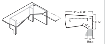
Extended Corner Island Faux Pedestal and Post - LEFT*
