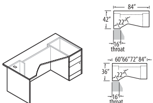
Single Pedestal Extended Corner Desk - RIGHT
