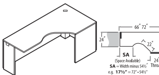
Extended Corner, 24" Throat - RIGHT
