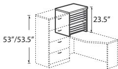
Transitional Pigeon-Hole Storage 23.5" High*
