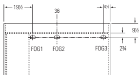
36 x 72 single pedestal left desks (A3672SPL)
