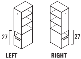
66" H Recycling Cabinet w/Bookshelf at 27" H
