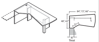
Extended Corner Island Faux Pedestal and Post - RIGHT*
