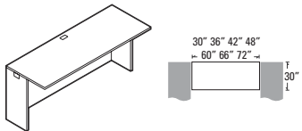
30" Deep Connectable Table
