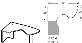
Extended Corner Island - RIGHT*
