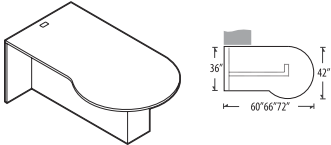
"P" Island LEFT - Full Modesty Panel (H-Base)*
