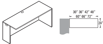
24" Deep Connectable Table - RIGHT
