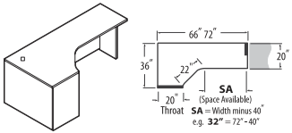
Extended Corner, 20" Throat - LEFT
