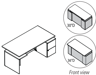
Single Pedestal Desk for Height Adj. Base*
