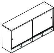
Overhead Storage, Sliding Glass Doors with Pigeon Hole - 32.5"/33"H
