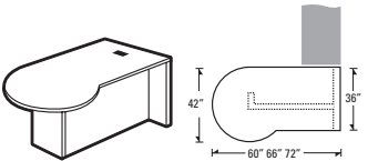
"P" Island - Full Modesty Panel (H-Base) - RIGHT
