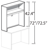
Open Hutch with Closed Back 42.4" High
