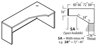
Extended Corner, 16" Throat - RIGHT
