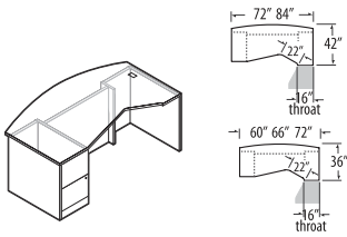
Single Pedestal Bow Top Extended Corner Desk - LEFT
