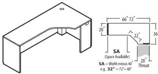
Extended Corner, 20" Throat - RIGHT
