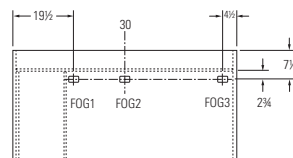
30 x 60 single pedestal left desks (G3060SPL)
