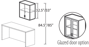
Closed Front Overhead Storage with Doors - 33"/33.5" High*
