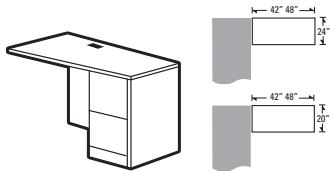
Full to Floor Flush Return - RIGHT*
