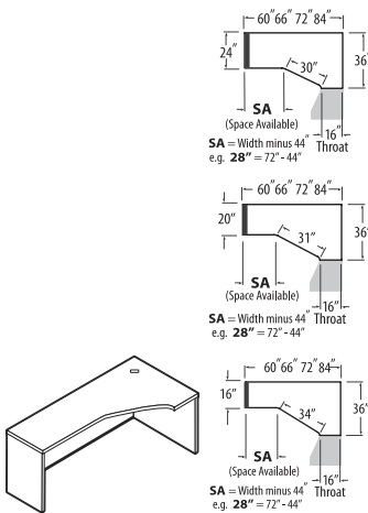
Extended Corner, 16" Throat - RIGHT
