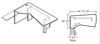
Extended Corner Island Faux Pedestal and Post - RIGHT*
