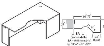
Extended Corner, 24" Throat - RIGHT
