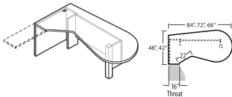
Extended Corner "P" Island Faux Pedestal and Post - RIGHT
