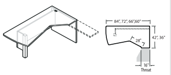
Extended Corner Island Recessed Modesty and Post - LEFT*
