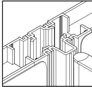
"T" (uneven height) "X" uneven height requires one more filler profile
