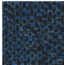
II12 Ozone
