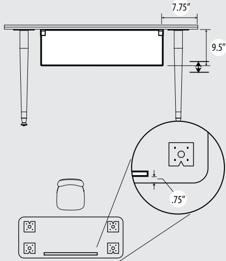
Square Modesty Panel
