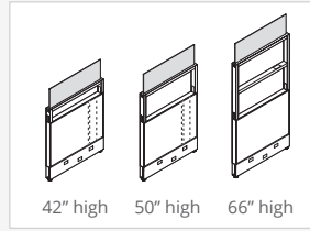
Pass-thru panel with vertical wire channel and embedded felt divider - fabric base
