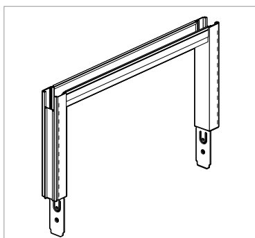
Overpanel frame is enclosed on both sides with laminate, fabric, or accessory tiles—or on one side with glass tile
